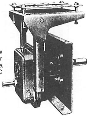
Flange mounted drive, Type JF
